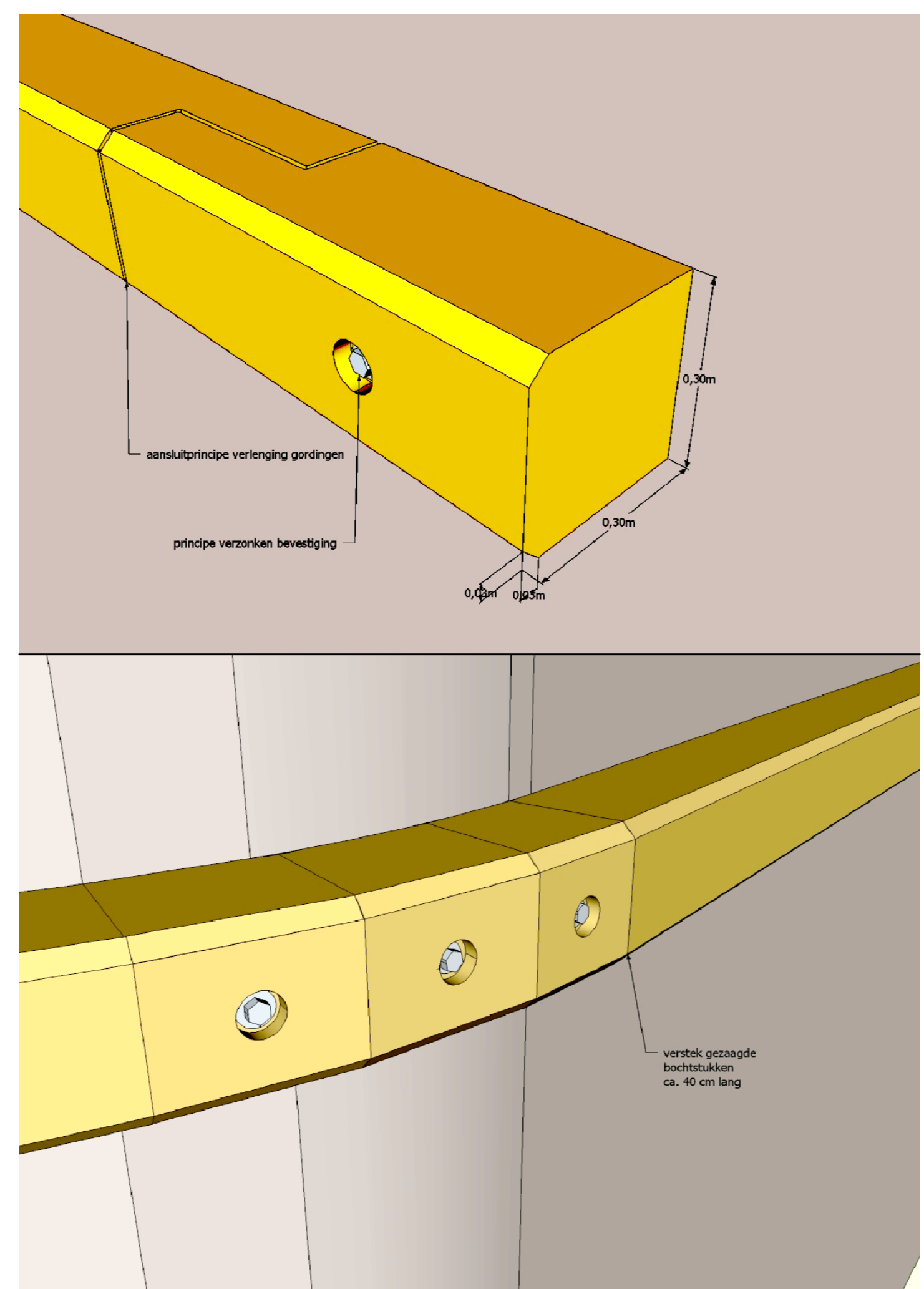
PRINCIPE-DETAILS GORDING
